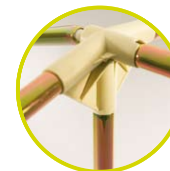
Corner joint > in reinforced plastic material
